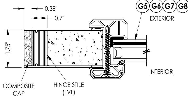
3 3 HORIZONTAL CROSS SECTION
