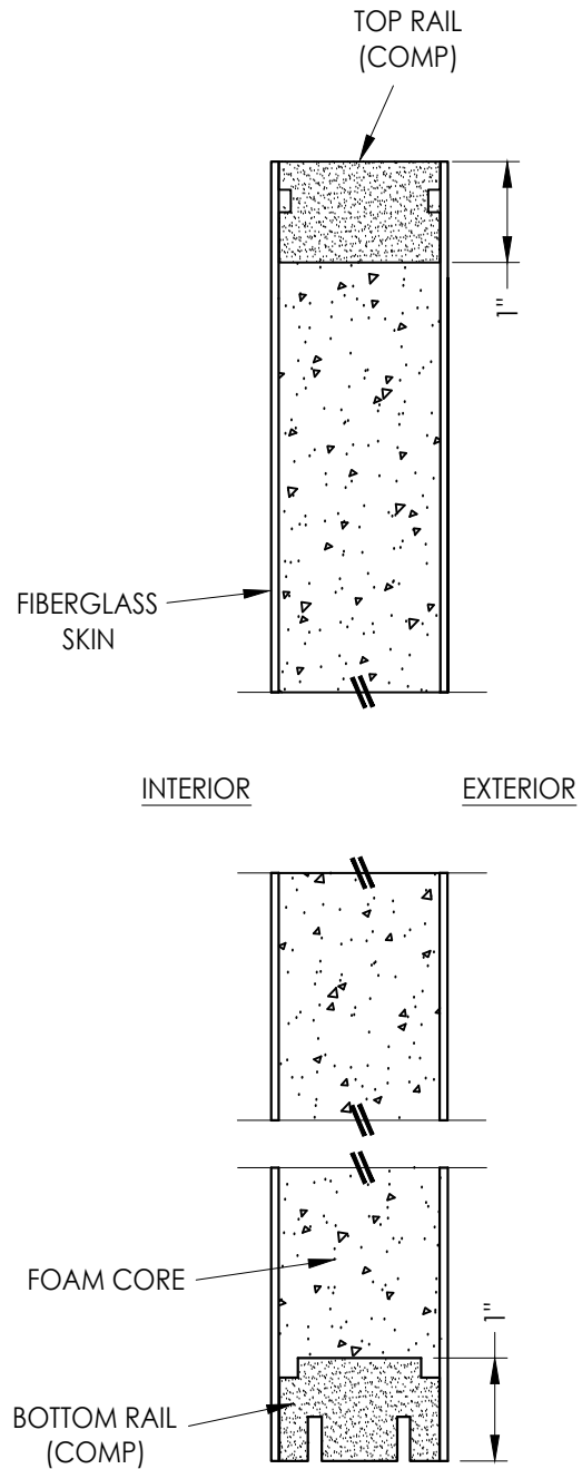
2 VERTICAL CROSS SECTION 2
