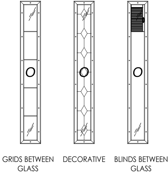
ALTERNATE GLAZING DETAILS
