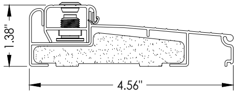
14 INSWING ADJUSTABLE THRESHOLD ZAILAA4565
