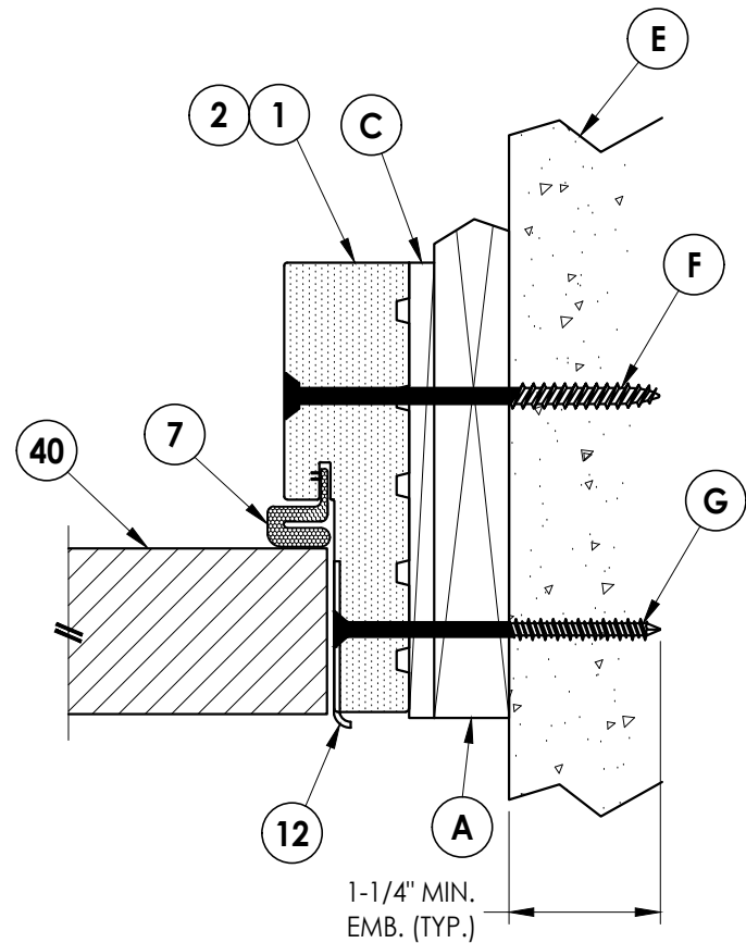
2 HORIZONTAL CROSS SECTION 9 Outswing Shown (Inswing Similar) Shown w/ 1X Buck
