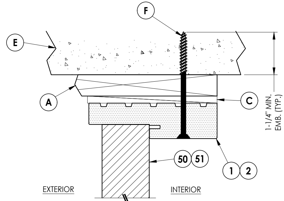
5 VERTICAL CROSS SECTION 9 Outswing Shown (Inswing Similar) Shown w/ 1X Buck
